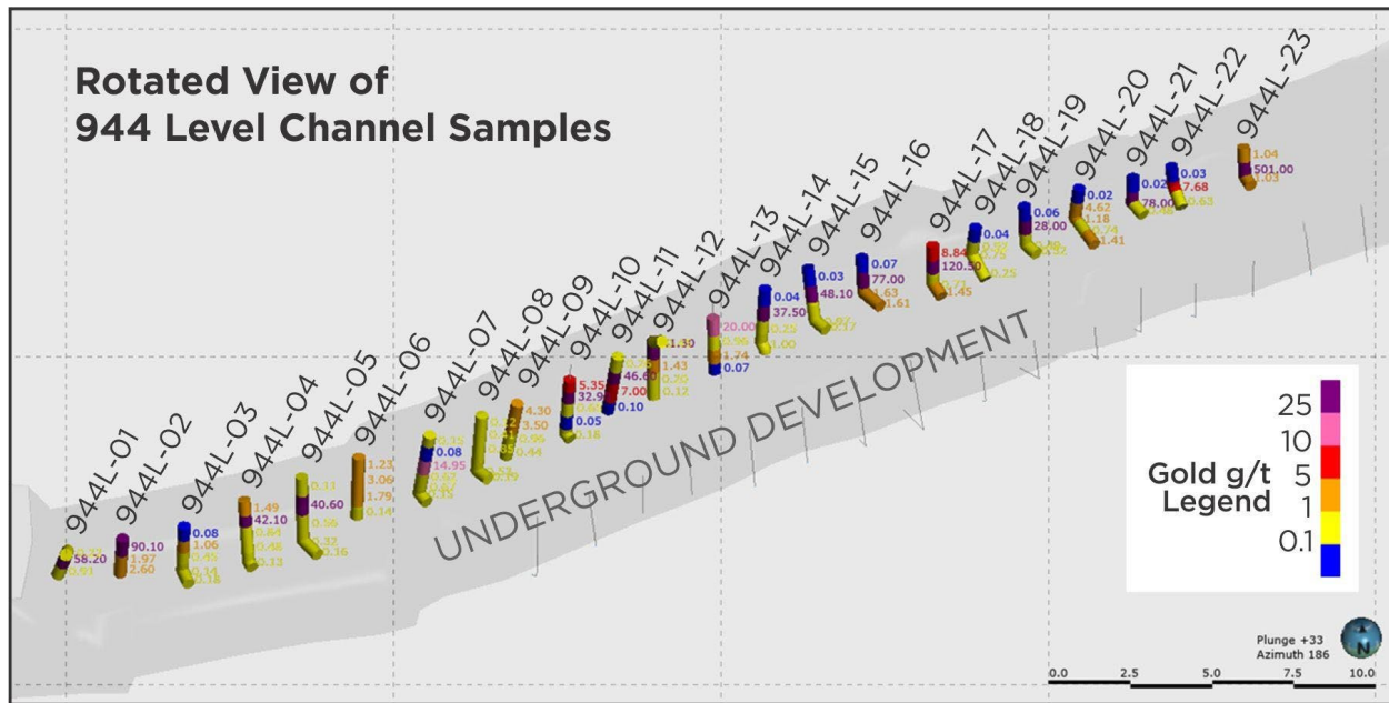
Figure 1. Section showing 944 Level Channel sampling program
