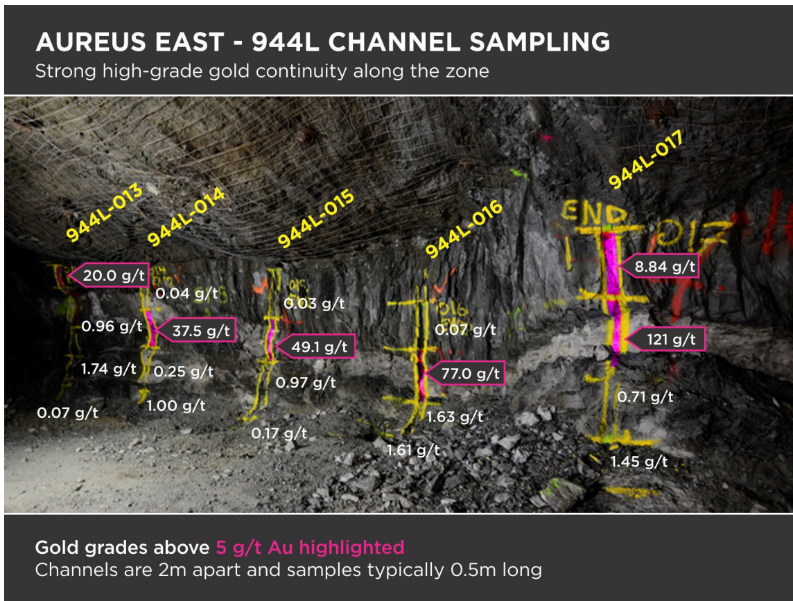
Figure 3. Photo of underground channel sampling program on 944L looking to the west.
