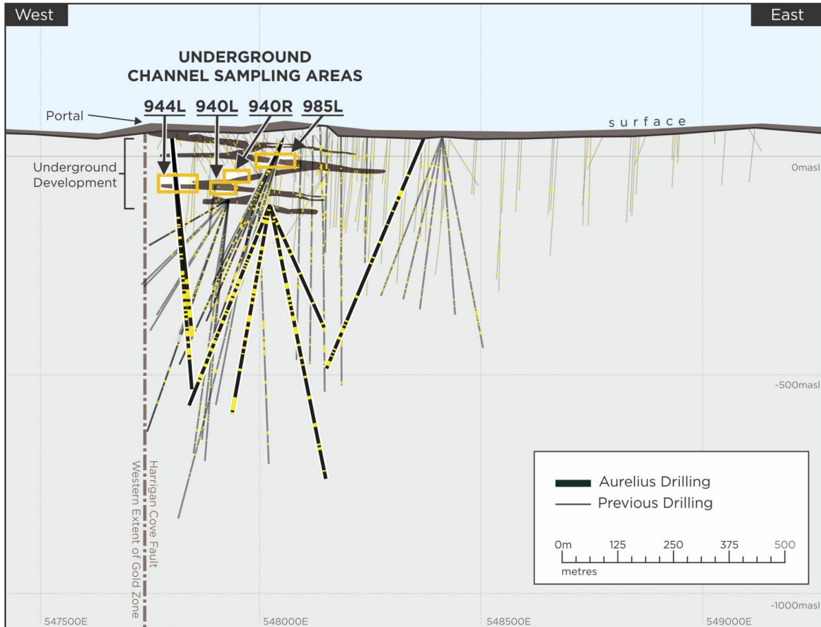
Figure 2. Long section showing locations of channel sampling programs
